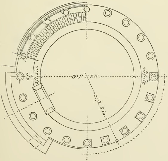
GROUND-PAN AND ELEVATION OF THE TEMPLE OF VESTA (restored).
